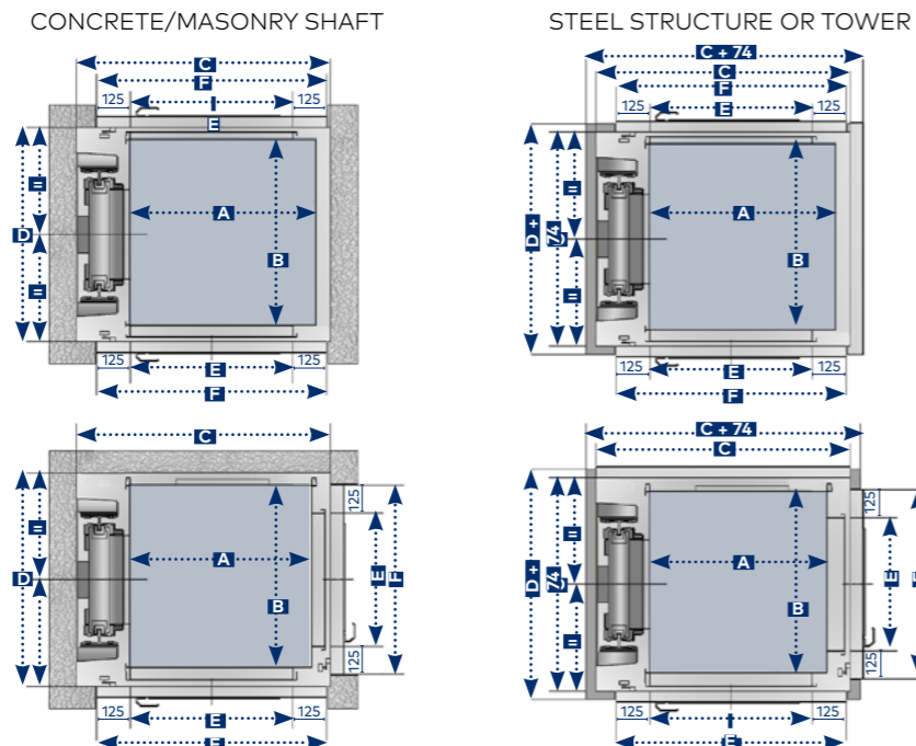
ALL DIMENSIONS EXPRESSED IN MILLIMETRES
